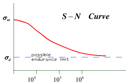
Fig. 1 Fatigue of ductiles
